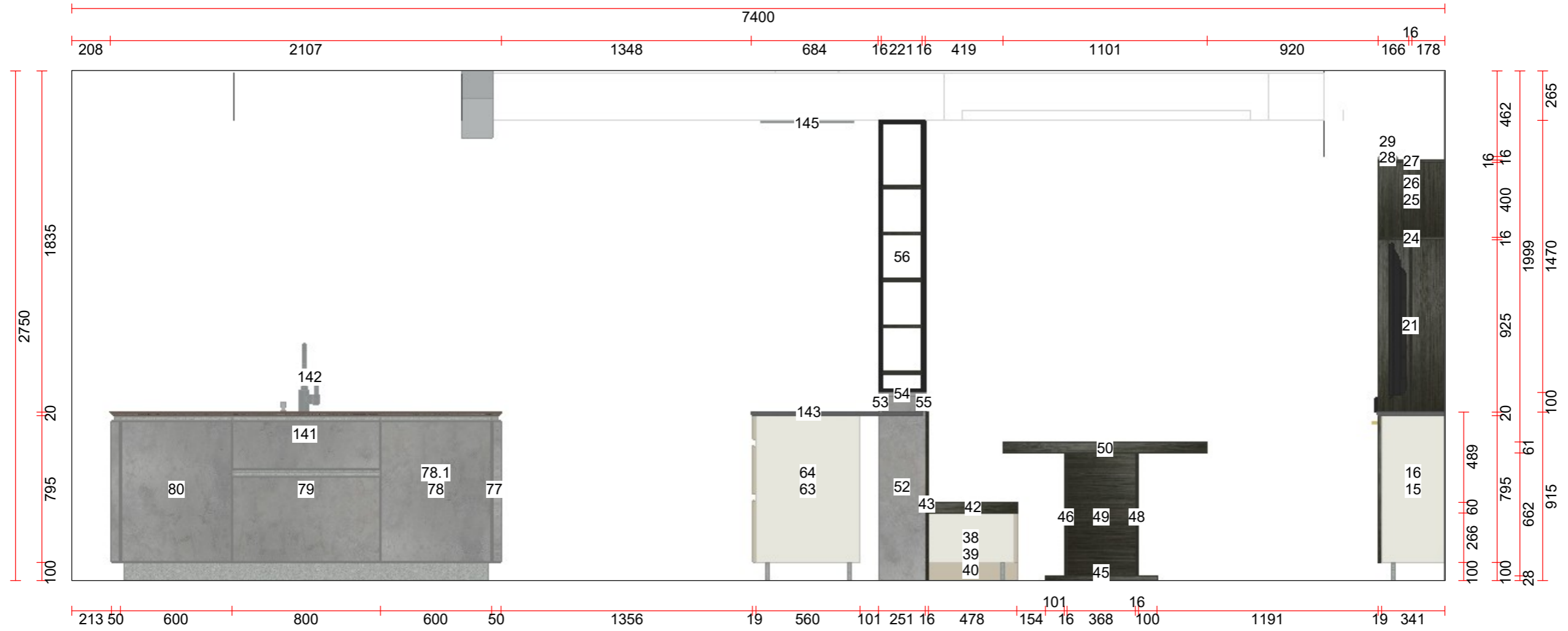
Elevation C
