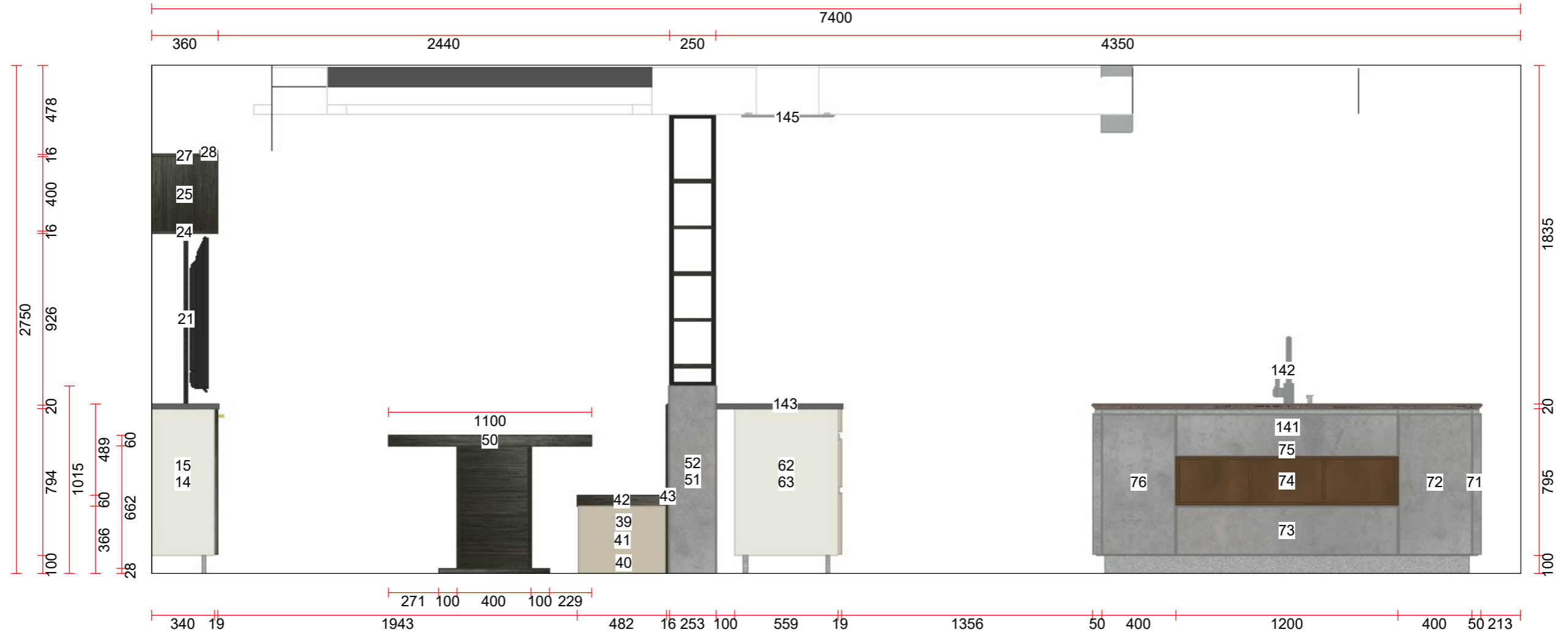
Elevation D
