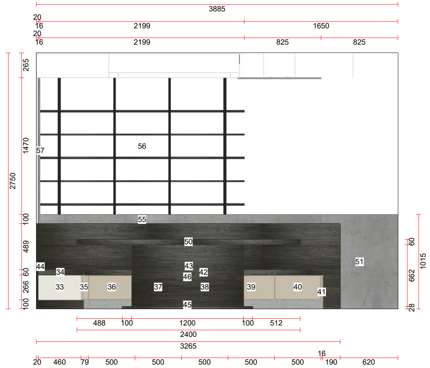
Elevation F
