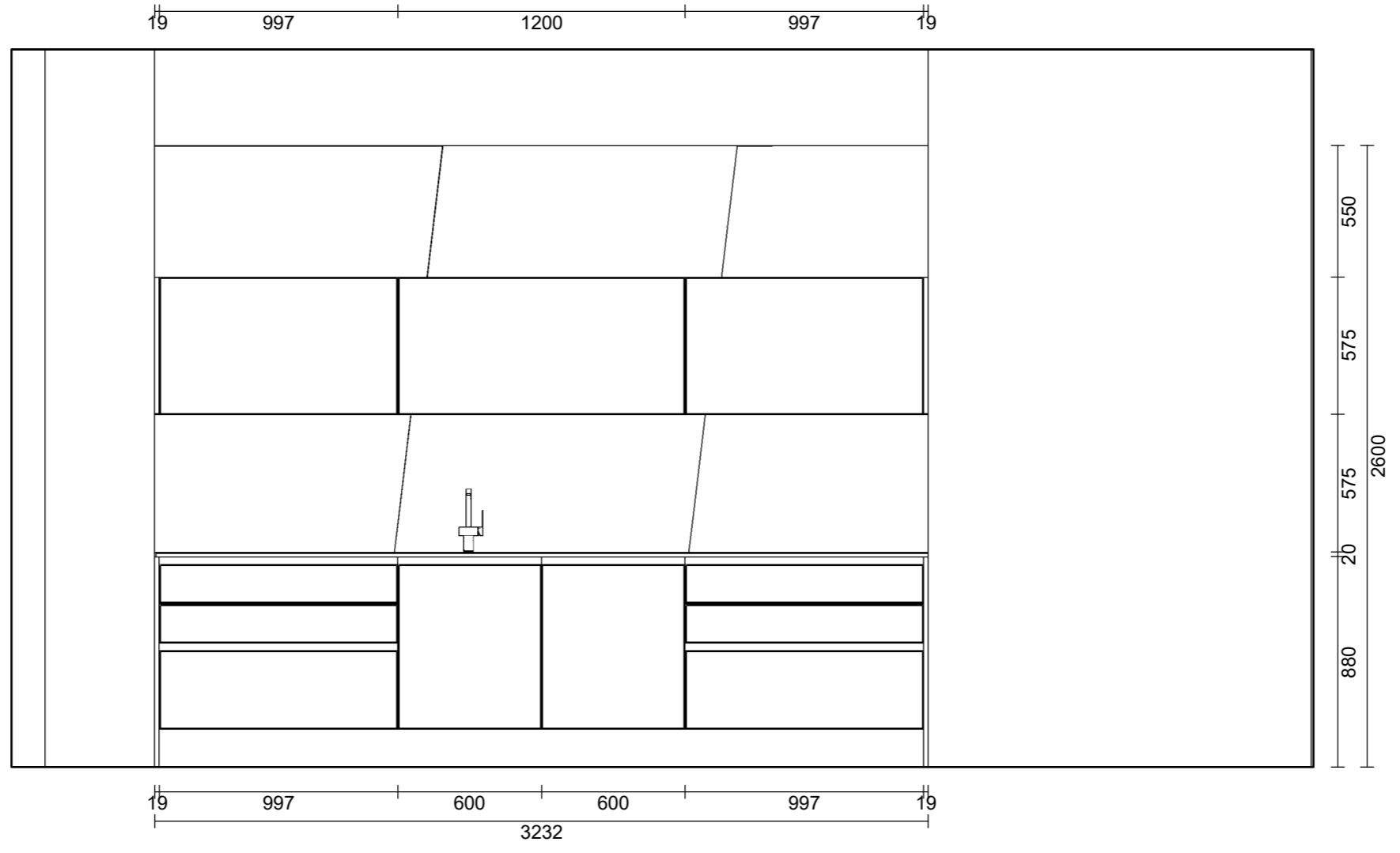
Elevation B/B
